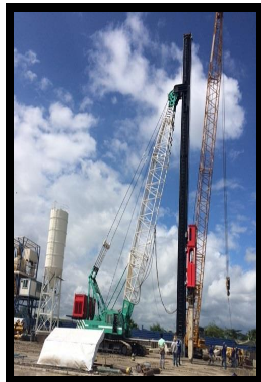
HYDRAULIC / DIESEL HAMMER
